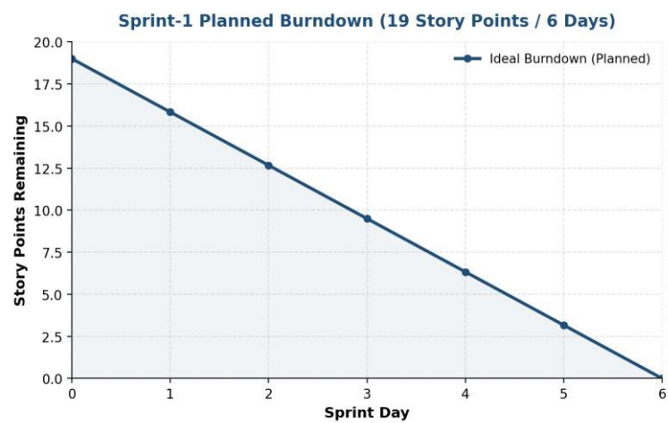
Figure 5.1: Sprint-1 Planned Burndown
