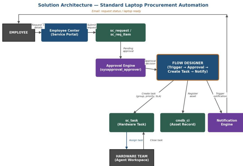
Figure 4.1: Solution Architecture — Standard Laptop Procurement Automation
